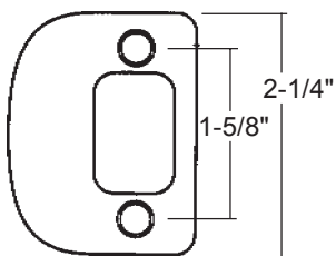
KW-85303 US-10B, 15, 15A Deadbolt strike with lip. 1/4" radius corners.
