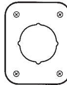
DJ-RP13545 Finishes: 605, 609, 630. Size: 3-1/2" x 4-1/2"
