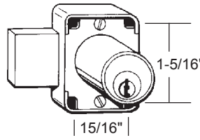
Pin Tumbler 0737 7/8 KA KA# B4R37539
