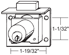
Pin Tumbler 0666 7/8 KA KA# 4T37526
