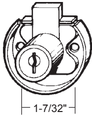
Disc Tumbler 02068 7/8" Deadbolt 02068 1/2-7/8" Latchbolt KD only
