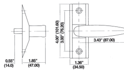
Thumbturn Cylinder
